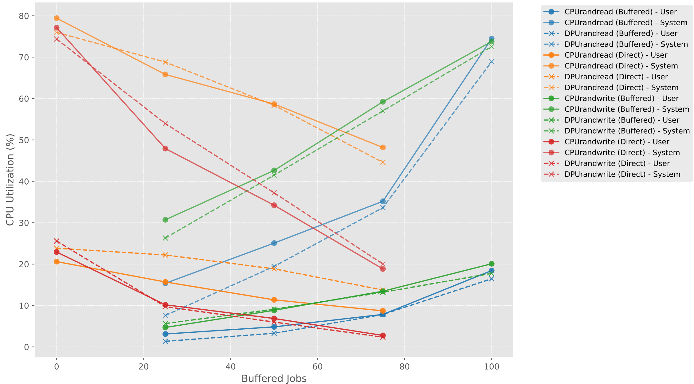
CPU Utilization vs Buffered Jobs (mixed) - RAND (CPU vs DPU)
